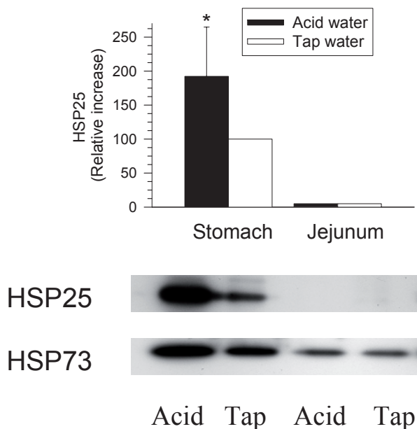
Fig. 1 Percentage increase in HSP protein expression in mice drinking acid water compared to tap water. HSP 25 and HSP73 protein levels were assessed by immunoblot analysis in mucosal samples of the stomach and jejunum in mice drinking either acid or tap water for 8 weeks. HSP values are expressed as relative changes between mice drinking tap water and acidified water using the ratio of HSP25 to the constitutively expressed HSP73. HSP25 expression was significantly increased (*: P < 0.05 , paired t test, n=7 ) approximately 2 fold in the stomach of mice drinking acid water. As previously reported, the jejunum did not express HSP 25.
