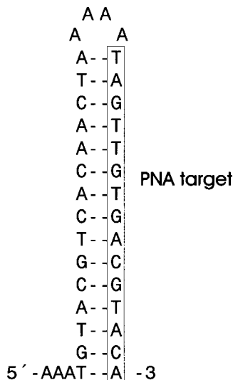
Figure 1. Sequence and predicted secondary structure of the 37 mer synthetic target oligonucleotide.
