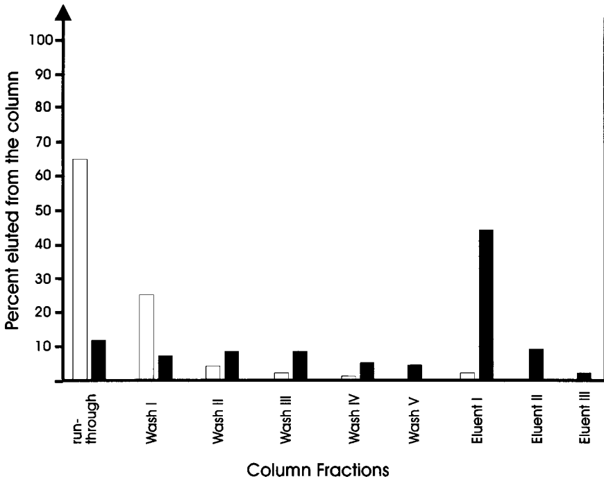
Figure 2. Capture efficiency of the hairpin oligonucleotide depicted in Figure 1 as a function of the ionic strength of the hybridization buffer. The radioactivity in each of the fractions is represented as the percentage of total radioactivity in all fractions. White bars: High salt, Black bars: Low salt.
