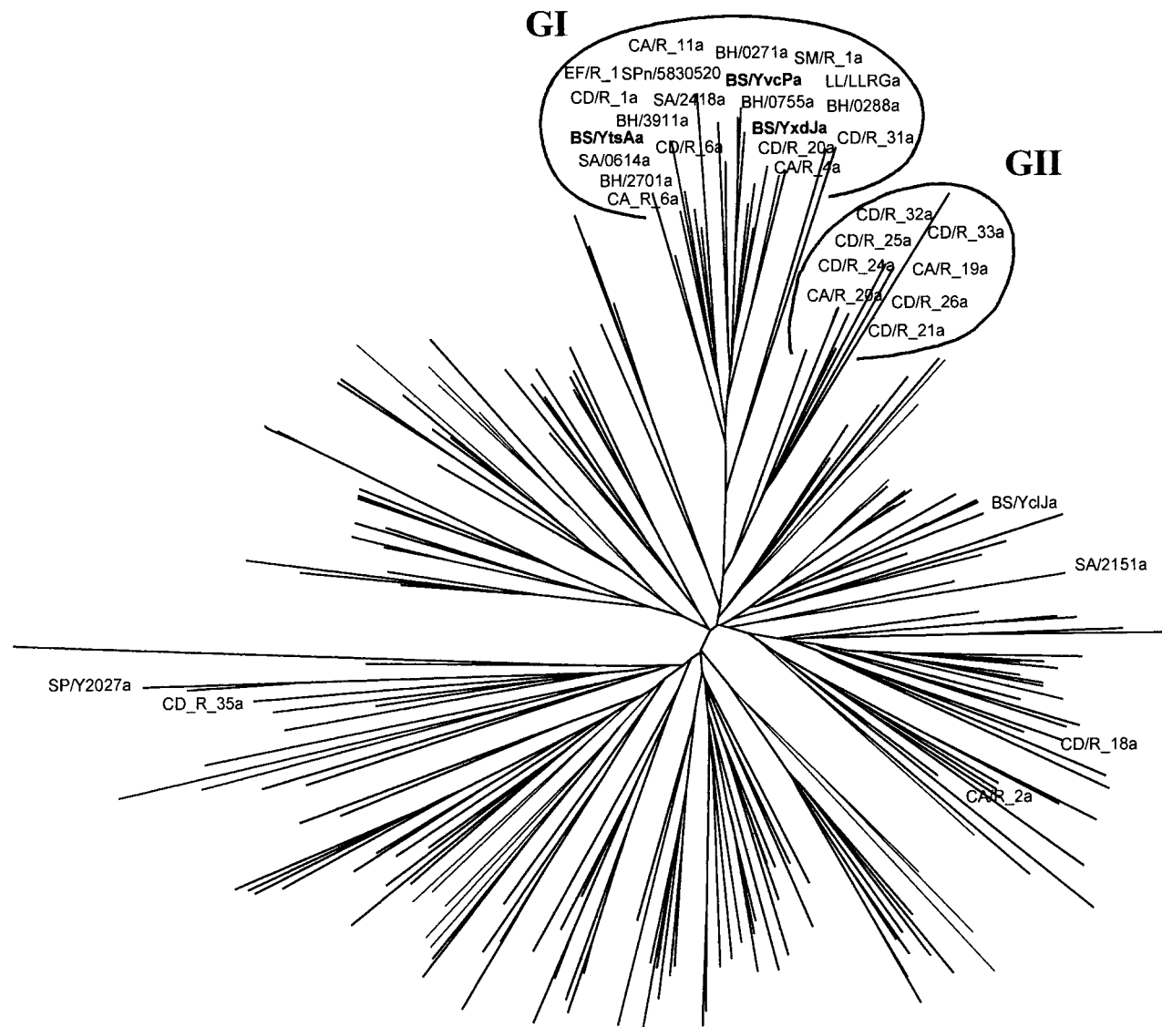
Figure 2. Unrooted tree of the OmpR family response regulators. The branch lengths are proportional to the evolutionary distances. To simplify the figure, RRs are included only if they have interesting characteristics and are discussed in the text. The letter 'a' at the end of the name indicates that RR is encoded by gene clustered with NBD genes. R, response regulator; BS, Bacillus subtilis ; BH, Bacillus halodurans ; CA, Clostridium acetobutylicum ; CD Clostridium difficile ; EF, Enterococcus faecalis ; LL, Lactococcus lactis ; SA, Staphylococcus aureus ; SM, Streptococcus mutans ; SPn, Streptococcus pneumoniae ; SP, Streptococcus pyogenes .
