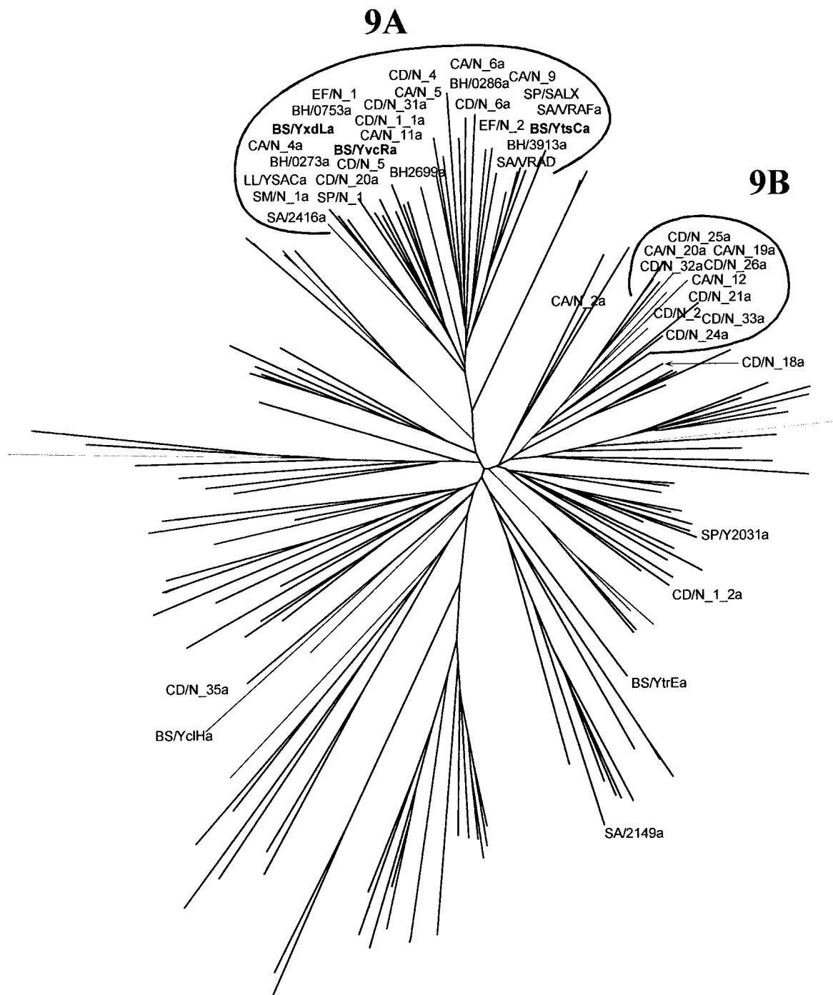
Figure 3. Unrooted tree of the Nucleotide Binding Domains from sub-family 9. The branch lengths are proportional to the evolutionary distances. Group "9A" is supported by a bootstrap value of 70%. To simplify the figure, NBDs are included only if they have interesting characteristics and are discussed in the text. The letter 'a' at the end of the name indicates that NBD is encoded by gene clustered with TCS genes. N, NBD; BS, Bacillus subtilis ; BH, Bacillus halodurans ; CA, Clostridium acetobutylicum ; CD Clostridium difficile ; EF, Enterococcus faecalis ; LL, Lactococcus lactis ; SA, Staphylococcus aureus ; SM, Streptococcus mutans ; SPn, Streptococcus pneumoniae ; SP, Streptococcus pyogenes .
