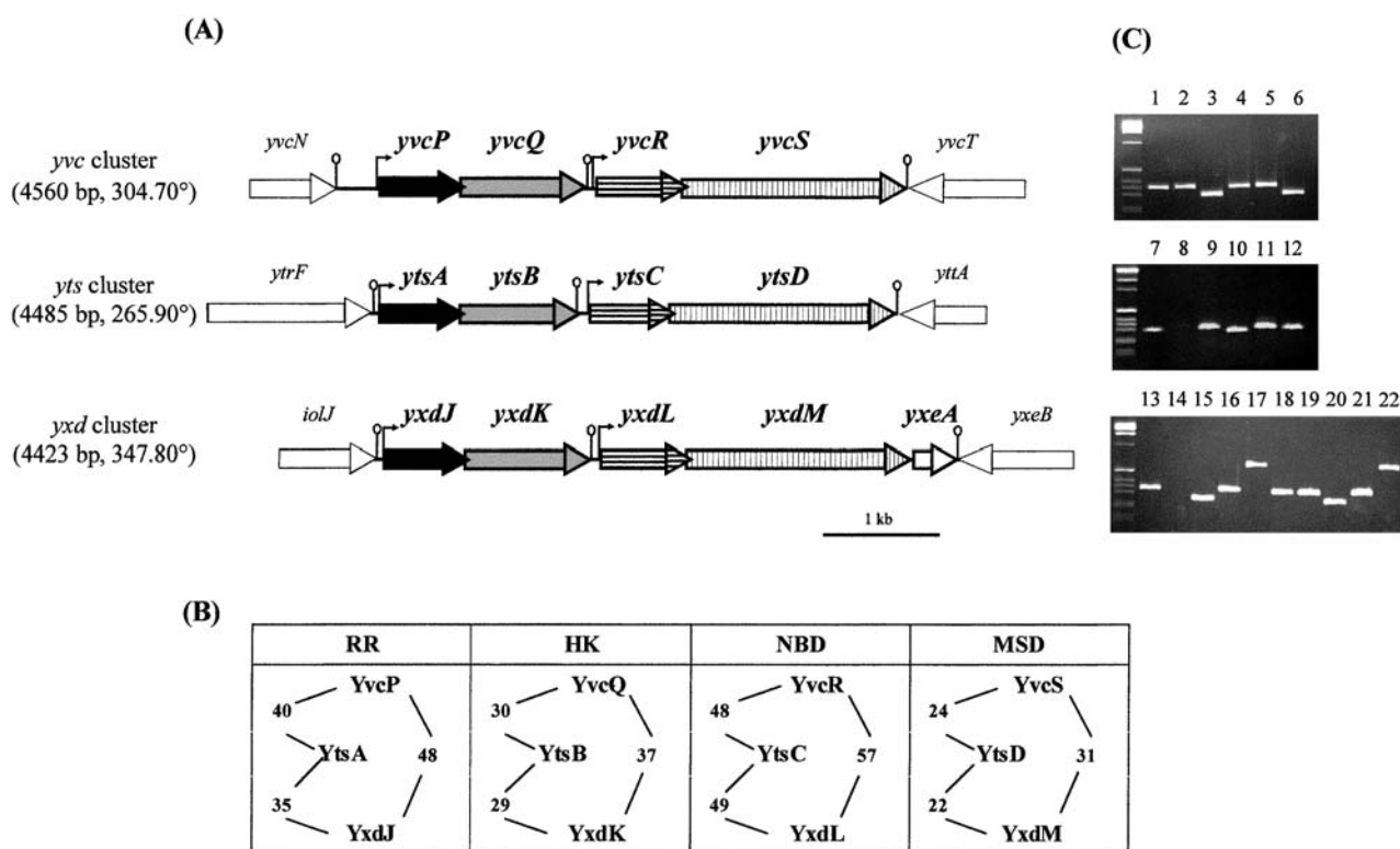
Figure 1. The three related clusters yvc , yts and yxd in B. subtilis . (A) Schematic representation of the three clusters. Black arrows correspond to RR genes, grey arrows to HK genes, horizontally hatched arrows to NBD genes and vertically hatched arrows to MSD genes. The position of putative promoters and terminators are indicated. The size of the clusters and their location on the chromosome are given between brackets. Upstream of yvcP is the crh -containing operon (Galinier et al. , 1997), upstream of ytsA is the ytr operon involved in acetoin utilisation (Yoshida et al. , 2000b) and upstream of yxdJ is the iol operon involved in myo -inositol catabolism (Yoshida et al. , 1997). Only the last genes in these operons are represented. (B) Identity scores obtained when comparing the functional related proteins are indicated and expressed as percentages. Similarity searches were done with the gapped version of the BLASTP2 program suite (Altschul et al. , 1997). In order to simplify the table, BS/ was omitted in protein names. (C) PCR products generated by RT-PCR. Ethidium bromide-stained 2% agarose gels of PCR products obtained with primers spanning the intergenic region between HK and NBD genes (lanes 2, 5, 8, 11, 14 and 19) and yxdM - yxeA (lanes 17 and 22), products obtained with specific primer of individual HK genes (lanes 1, 4, 7, 10, 13 and 18), NBD genes (lanes 3, 6, 9, 12, 15 and 20) and MSD gene (lanes 16 and 21). Templates for PCR were: cDNA prepared from B. subtilis 168 total RNA (lanes 1 to 3; 7 to 9; 13 to 17); B. subtilis 168 chromosomal DNA (lanes 4 to 6; 10 to 12; 18 to 22). No PCR product with RNA as template was obtained (not shown).
