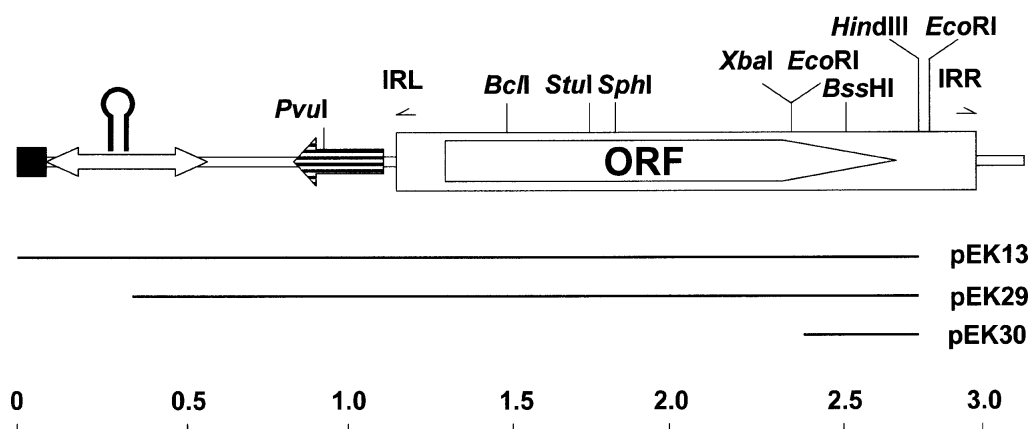
Figure 1. Diagram of the chromosomal region adjacent to the Tn1545 insertion point in strain C10. The end of Tn1545 (filled box), a region able to form a stable secondary structure (double headed arrow), and the sinR -like gene (arrow) are shown, as is the IS (open box) together with its associated ORF and terminal inverted repeats (IRL and IRR). The positions of landmark restriction sites are indicated, as are the inserts cloned in plasmids pEK13, pEK29 and pEK30. The scale below the diagram is in kbp.
