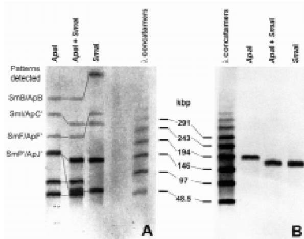
Figure 4. Detection of ISCb1 in Apal and SmaI macro-restriction fragments from C. beijerinckii DNA. Macro-restriction fragments were prepared from strains NCIMB 8052 (Part A) and C10 (Part B) as described previously (Wilkinson and Young, 1995). An ISCb1-specific probe (pEK30) was employed in part A and an aphA -3-specific probe (see Experimental procedures) in part B. Bands corresponding to macro-restriction fragment profiles that had been identified previously (Wilkinson and Young, 1995) are indicated. Note that the SmP'/ApJ' profile detected in part B has been shifted relative to its counterpart in part A, owing to the presence of a copy of Tn1545 (25.3 kbp - Caillaud et al. , 1987a) in the hybridising fragments.
