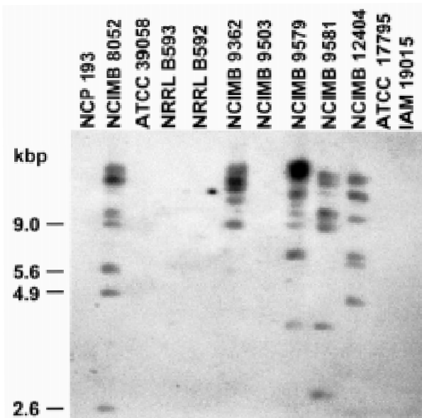
Figure 5. Distribution of ISCb1 among C. beijerinckii strains representing twelve different DNA fingerprint groups. DNA samples were digested with Bsp LU111, and probed with pEK30 DNA.
